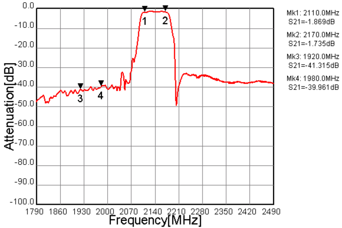
Fig.1 Pass-band Characteristic
